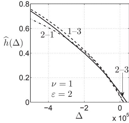
Figure 33: Robustness curves for comparing three options in eq.(293). Larger uncertainty weights.
