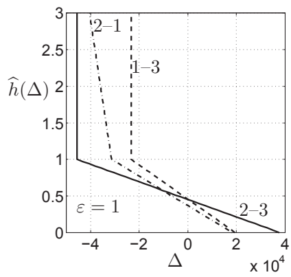
Figure 41: Robustness curves for comparing three options in eq.(293). Only WEI uncertainty and only for innovative sub-systems.
