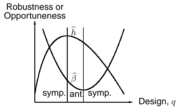
Figure 5: Robustness and opportunity curves which are both sympathetic and antagonistic.
