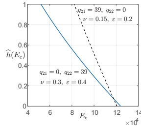
Figure 26: Robustness curves for the special case in eq.(264), with \tilde{v} and \tilde{W} in eqs.(253) and (254), and Q in eq.(255) modified as shown in the figure.
