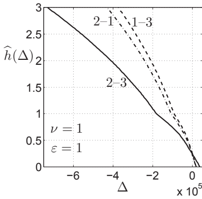
Figure 38: Robustness curves for comparing three options in eq.(293). Only WEI-WUV uncertainty.
