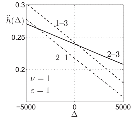
Figure 40: Same as fig. 38, expanded scale.
