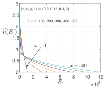
Figure 30: Robustness curves for the two APC options in eqs.(283)–(285).
