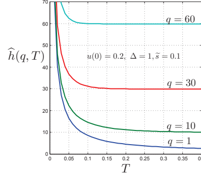
Figure 15: Robustness versus time, eq.(204), assuming u(0) < \Delta . The value of q increases from the bottom to the top curve.
