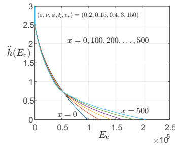
Figure 28: Robustness curves for the second example, with Q in eq.(282).
