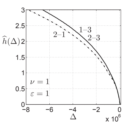
Figure 35: Robustness curves for comparing three options in eq.(293).
