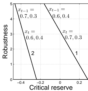
Figure 22: Robustness curves for two sequences of investments.
