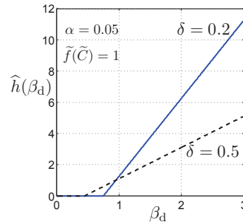
Figure 18: Innovation dilemma for choosing the effect size, \delta .
