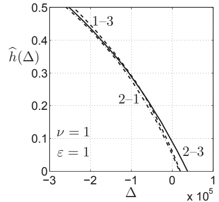
Figure 37: Same as fig. 35, expanded scale.
