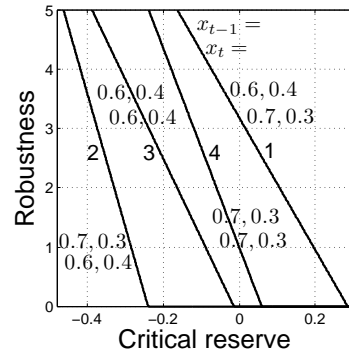
Figure 23: Robustness curves for 4 sequences of investments. Curves 1 and 2 reproduced from fig. 22.
