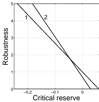
Figure 20: Robustness curves. x_{t-1} = x_t = (0.7, 0.3)^T . See table 1.
