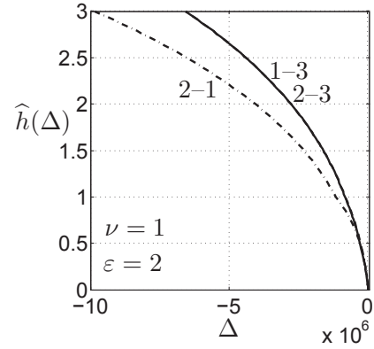
Figure 34: Same as fig. 33, reduced scale.
