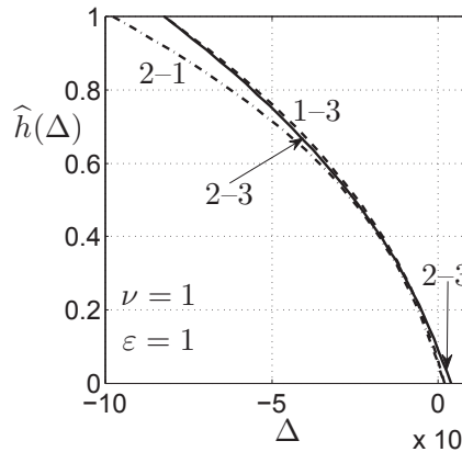
Figure 36: Same as fig. 35, expanded scale.
