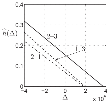
Figure 42: Robustness curves for comparing three options in eq.(293) with model uncertainty.
