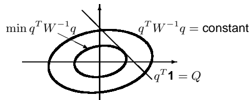
Figure 14: Schematic illustration of constrained optimization of q^T W^{-1} q .
