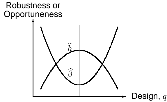
Figure 4: Sympathetic robustness and opportunity curves.
