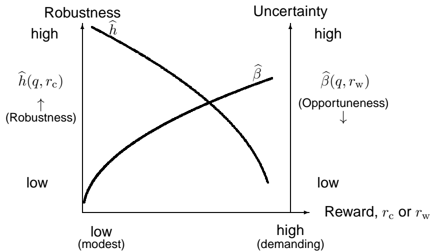
Figure 9: Robustness and opportuneness curves.
