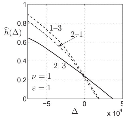
Figure 39: Same as fig. 38, expanded scale.
