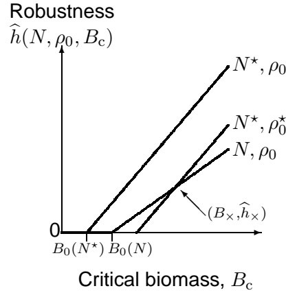
Figure 17: Robustness curves for N and N^* test points with trigger densities \rho_0 and \rho_0^* , eq.(213). N^* > N , \rho_0^* > \rho_0 .
