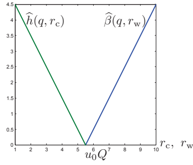
Figure 12: Trade off and zeroing for robustness and opportuneness. Eqs. (190) and (191).
