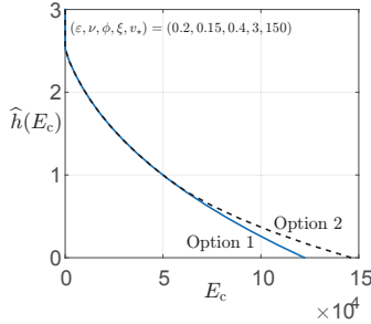
Figure 27: Robustness curves for the two options in eqs.(271)–(280).
