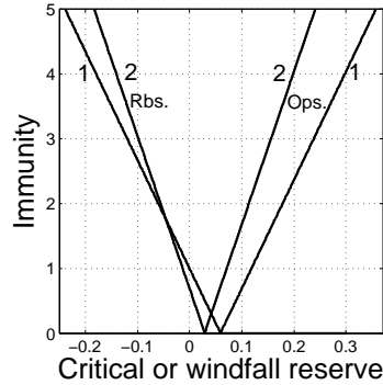
Figure 21: Robustness and opportuneness curves for portfolios in fig. 20.
