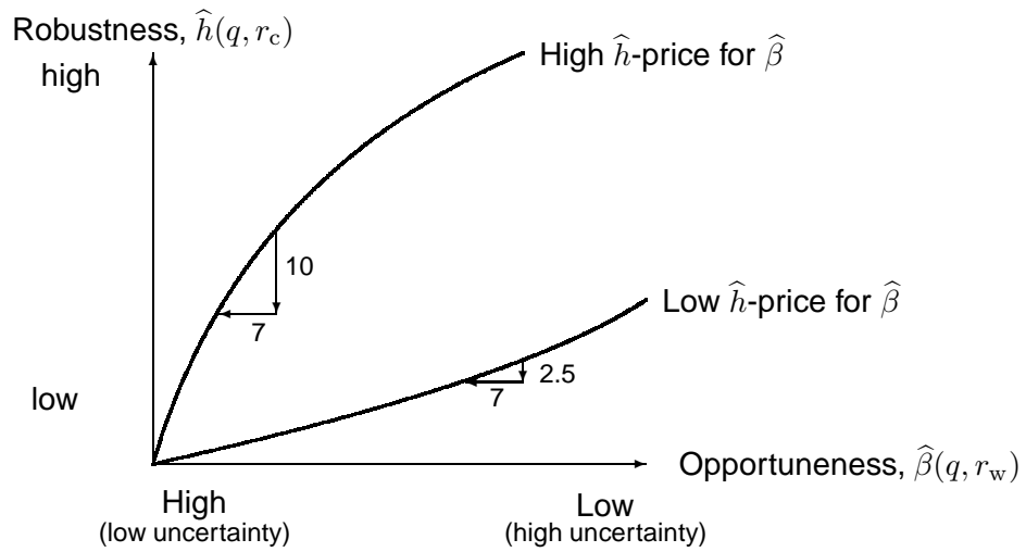
Figure 13: Trade-off between robustness and opportunity.
