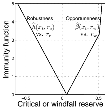
Figure 19: Robustness and opportuneness curves.
