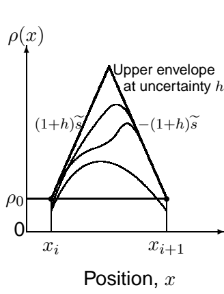
Figure 16: Evolution of M(h) , eq.(210), showing an upper envelope and three possible density curves.
