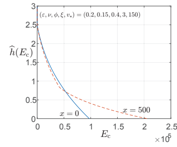
Figure 29: Robustness curves for the second example, with Q in eq.(282).
