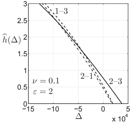
Figure 32: Robustness curves for comparing three options in eq.(293).
