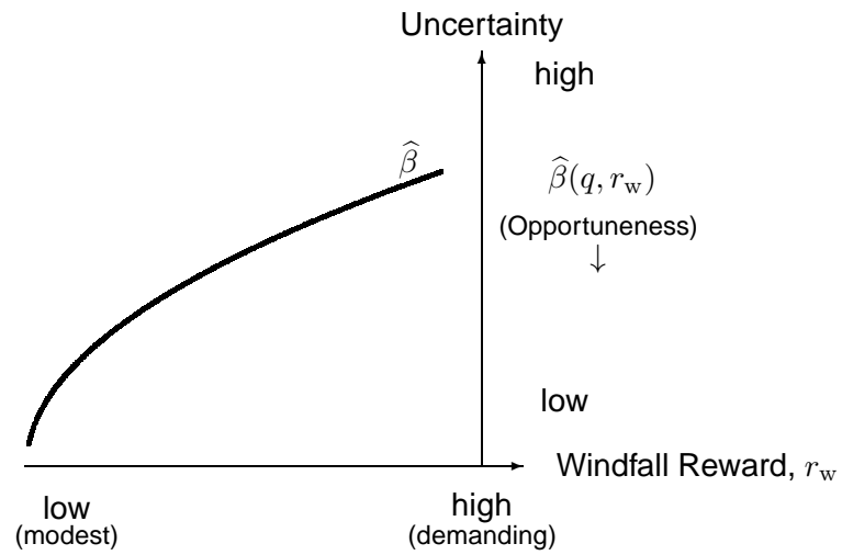
Figure 8: An opportuneness curve.
