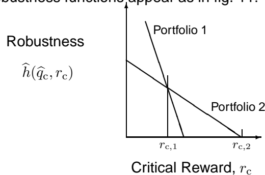
Figure 11: Robustness functions for two different portfolio investment alternatives.
