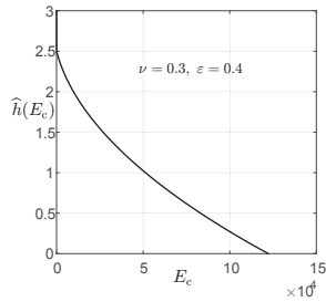
Figure 25: Robustness curve for the special case in eq.(264), with \tilde{v} , \tilde{W} and Q in eqs.(253)–(255).
